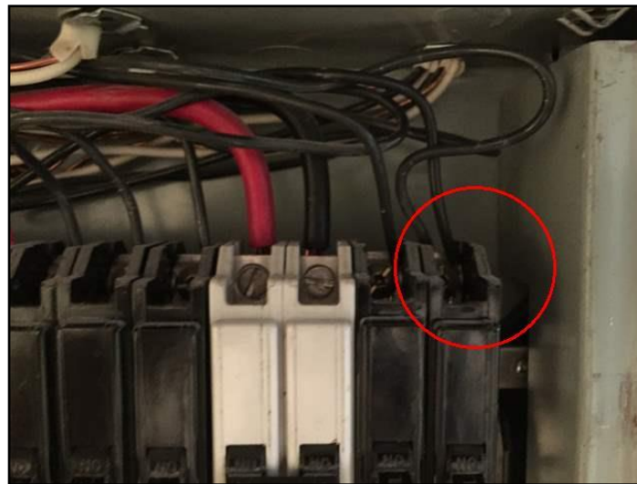
Double tap (two wires on one breaker or fuse)
